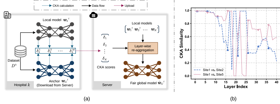
Fig. 1: (a) Overview of Fed-LWR. During the parameter aggregation stage of t -th round, Fed-LWR calculate layer-wise CKA similarity \delta_k = \{\delta_k^1, \delta_k^2, \dots, \delta_k^M\} between the local model w_k^t and anchor w_G^t averaged by server on hospital k . The CKA scores will be used to re-aggregate the local models to obtain fair global model \hat{w}_G^t . (b) Variations in CKA similarity versus the layers of local models from two pairs of clients, which are randomly selected. This reveals that the differences between models vary with different layers.
