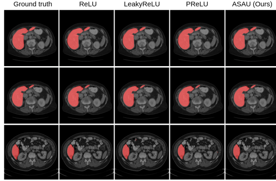
Fig. 4: Qualitative results comparison for liver segmentation results (LiTS) on the ResUNet++ model with various activation functions. It can be observed that ASAU produces more accurate segmentation maps in all three cases.
