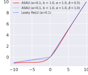
Fig. 2: Approximation of Leaky ReLU using ASAU for different values of a , b , \alpha , and \beta . As \beta \rightarrow \infty , ASAU smoothly approximates Leaky ReLU.
