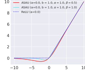
Fig. 3: Approximation of ReLU using ASAU for different values of a , b , \alpha , and \beta . As \beta \rightarrow \infty , ASAU smoothly approximates ReLU.
