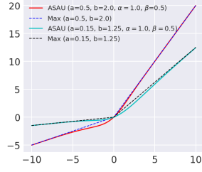
Fig. 1: Approximation of Maximum function using ASAU for varying values of a , b , \alpha , and \beta . As \beta \rightarrow \infty , ASAU smoothly approximates the maximum function.
