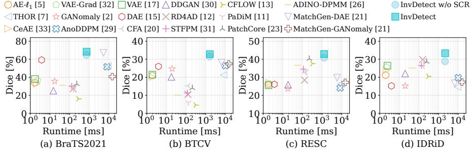
Fig. 2: The results of average runtime (milliseconds) vs. Dice. Reconstruction-based methods are shown by unfilled area-based markers (e.g., \square , \triangle , \star , etc). Embedding-based methods are shown by stroke-based markers (e.g., \times , + , etc).
