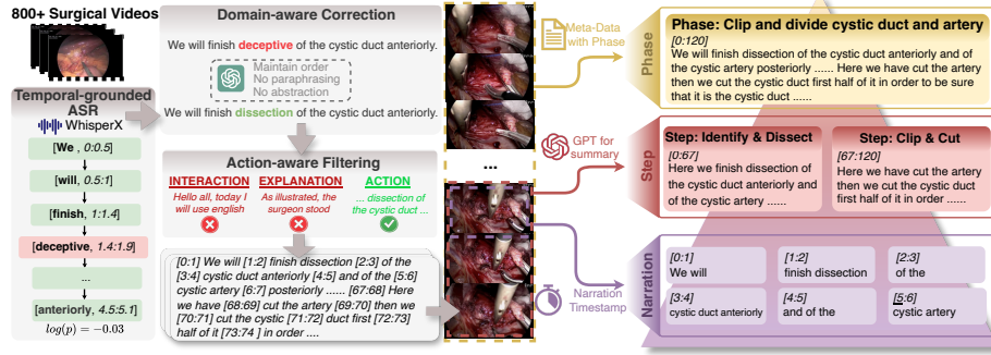
Fig. 1. Overview of the hierarchical temporal grounding pipeline for narration data curation.
